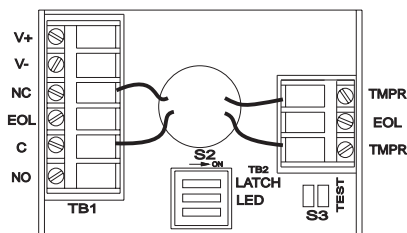
Figure 2 WIRING
